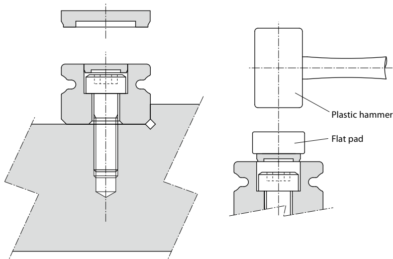
Fig.3 Cap for rail mounting hole
